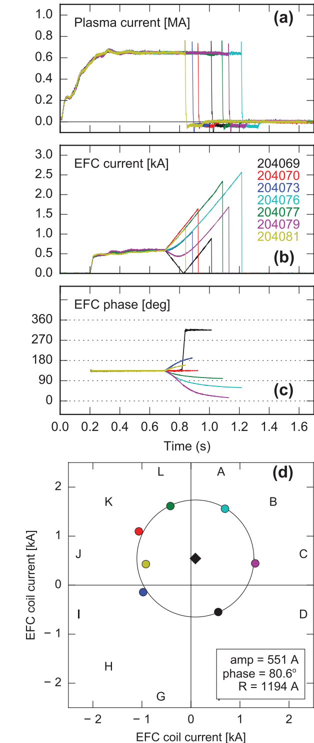
Figure 17. (a) Plasma current, (b) EFC coil currents, (c) phase of applied field from a sample compass scan, and (d) locking circle showing amplitude and phase of the EF.
