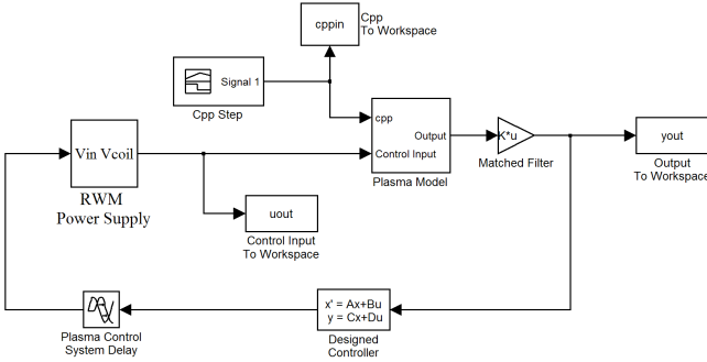
Fig. 5. Top Level of the Simulink model.
