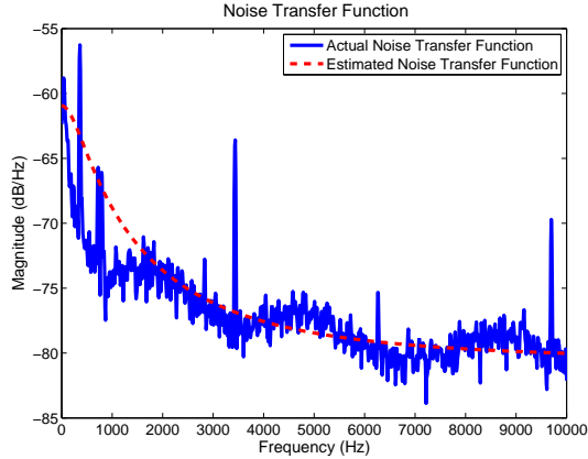
Fig. 4. Computed and estimated noise transfer function.
