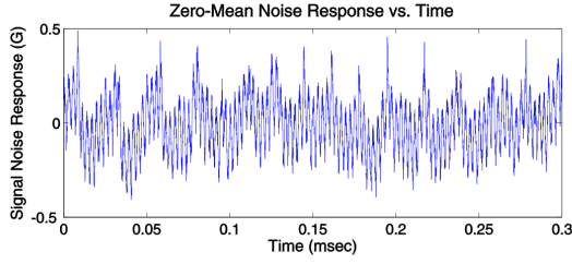
Fig. 3. Typical sensor noise signal in DIII-D.
