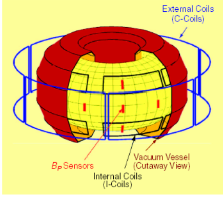
Fig. 1. Coils and sensors for RWM magnetic feedback stabilization.
