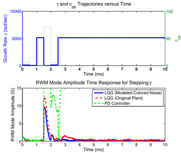
Fig. 8. Initial condition response control inputs for stepping \gamma .
