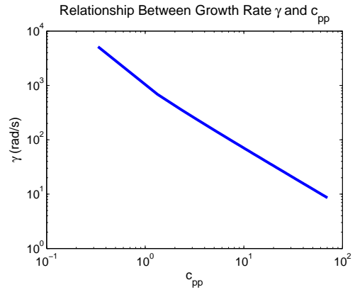
Fig. 2. Empirical relationship between the growth rate \gamma and c_{pp} .
