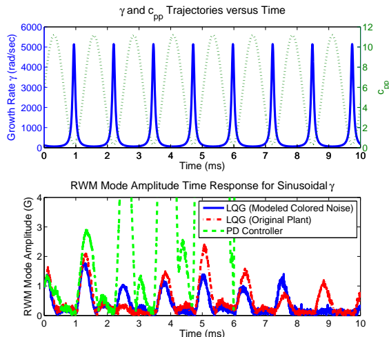
Fig. 9. Initial condition response control inputs for sinusoidal c_{pp} .
