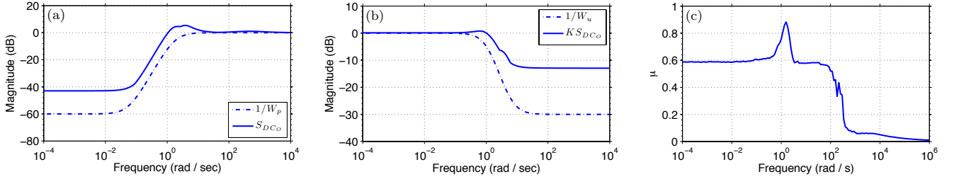
Fig. 4. Maximum singular values: (a) 1/W_p and S_{DCO} and (b) 1/W_u and KS_{DCO} and (c) \mu(N_{11}(j\omega)) versus frequency. The closed-loop robust stability condition is defined as \mu(N_{11}(j\omega)) < 1, \forall \omega (Skogestad and Postlethwaite (2005)).
