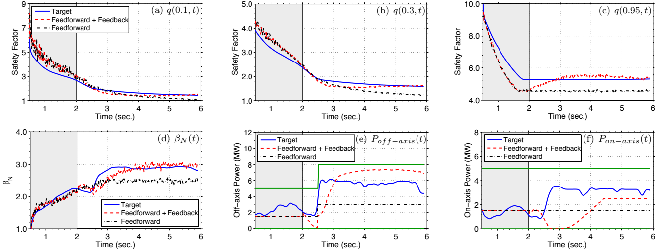
Fig. 5. Simulation testing of q -profile + \beta_N feedback controller: (a-c) time trace of q at various spatial locations, (d) time trace of plasma \beta_N , and (e-f) control actuator trajectory comparison (actuator limits in solid green). The gray-shaded region indicates when the feedback controller is inactive. Note gyrotrons become available at 2.5 sec.
