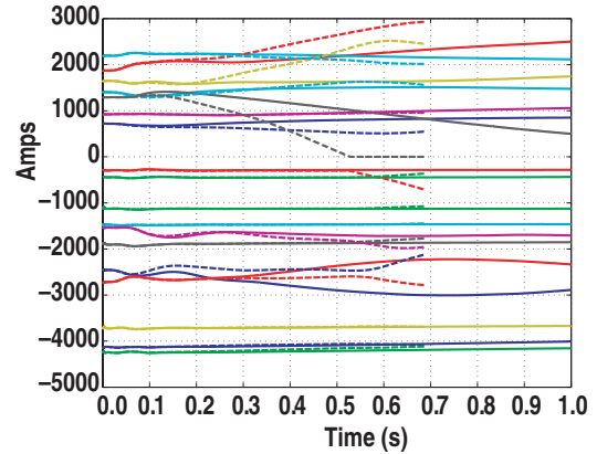
Fig. 6. Coil currents from simulations with (solid) and without (dashed) current limit prevention logic.
